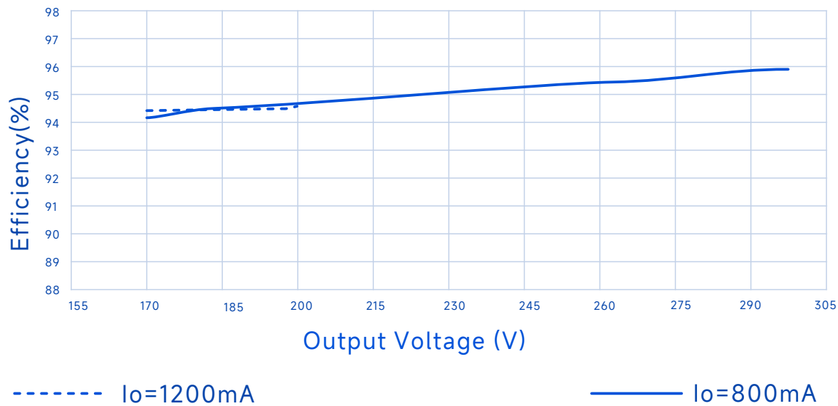
Efficiency Vs. Output Voltage (Vin=230Vac)
